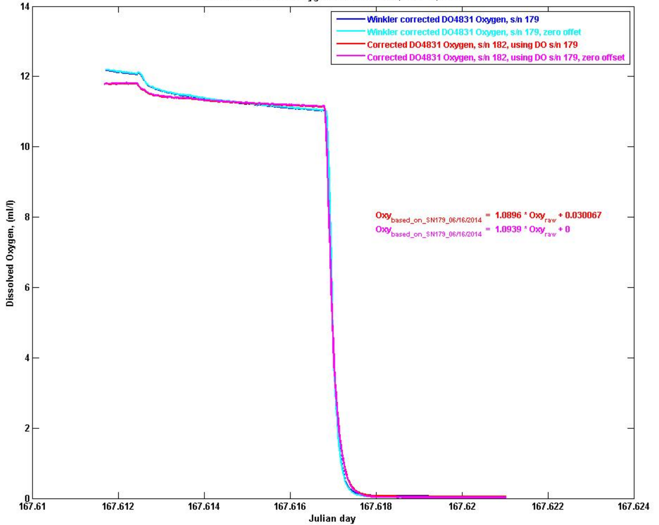
Corrected Dissolved Oxygen measurements, June 16, 2014
