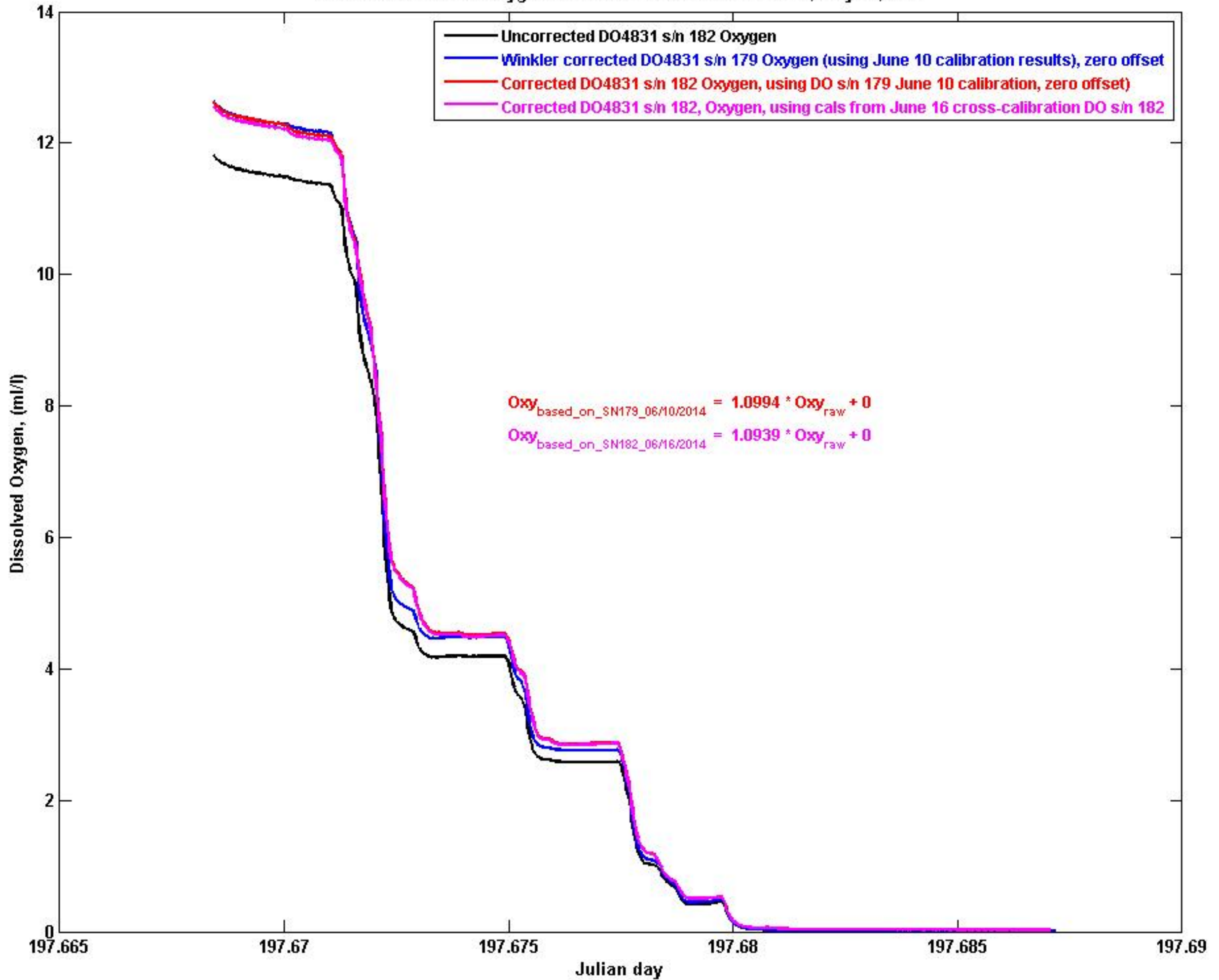
Corrected Dissolved Oxygen measurements DO4831 S/N 182, July 16, 2014
